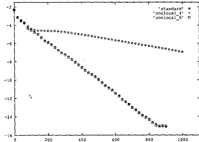
FIG. 4. Logarithm of \rho -residual in L_\infty -norm versus number of iterations; NACA0012, M_0 = 0.63 , \alpha = 2^\circ , Re = 400 , grid 192 \times 32 , “average radius” \approx 2 chords.
